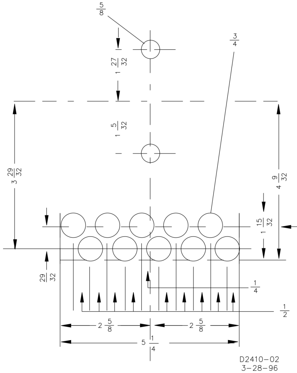
Figure 4-3. Panel Drilling Diagram for S1 Case, Projection Mounting
